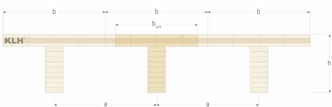
Fig. 5: Dimensions of the T-beam cross-section
